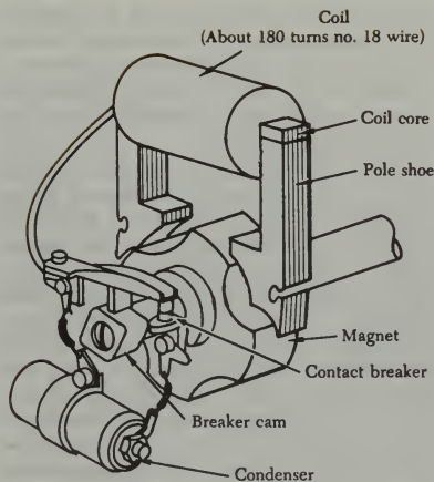
FIGURE 4-5. Components of a high-tension magneto circuit.
